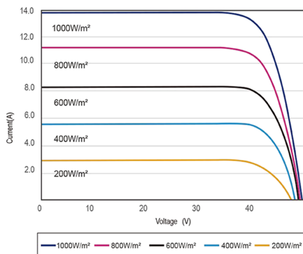
I-V CURVES OF PV MODULE(540W)
