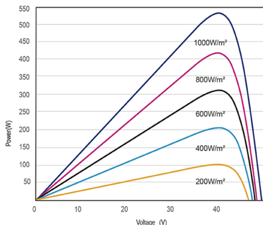
P-V CURVES OF PV MODULE(540W)
